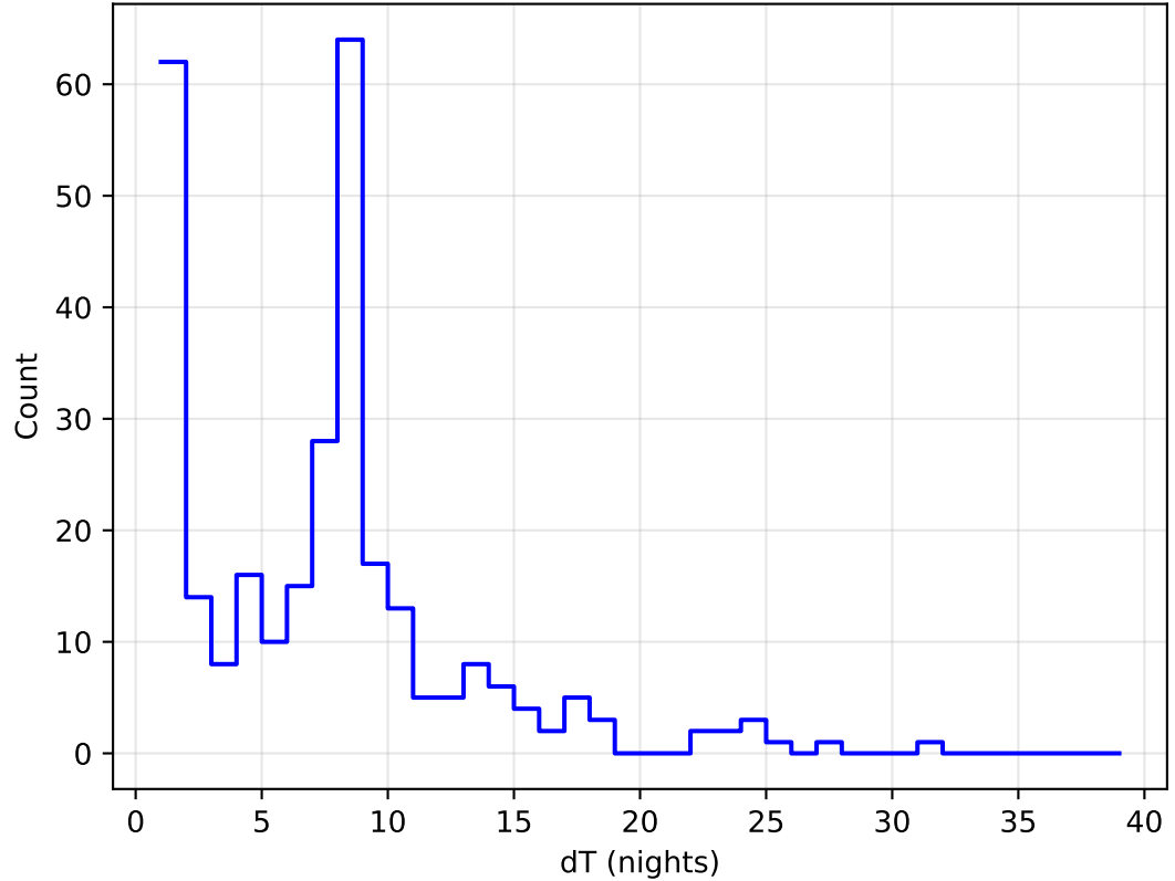
internal_u_expt60_nscale1.2v3.4_10yrs all bands: DD:XMM_LSS Delta Nights Histogram
