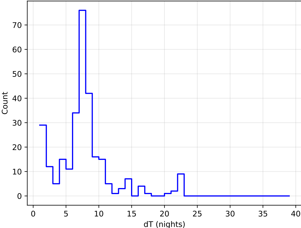
internal_u_expt60_nscale1.2v3.4_10yrs all bands: DD:EDFS Delta Nights Histogram
