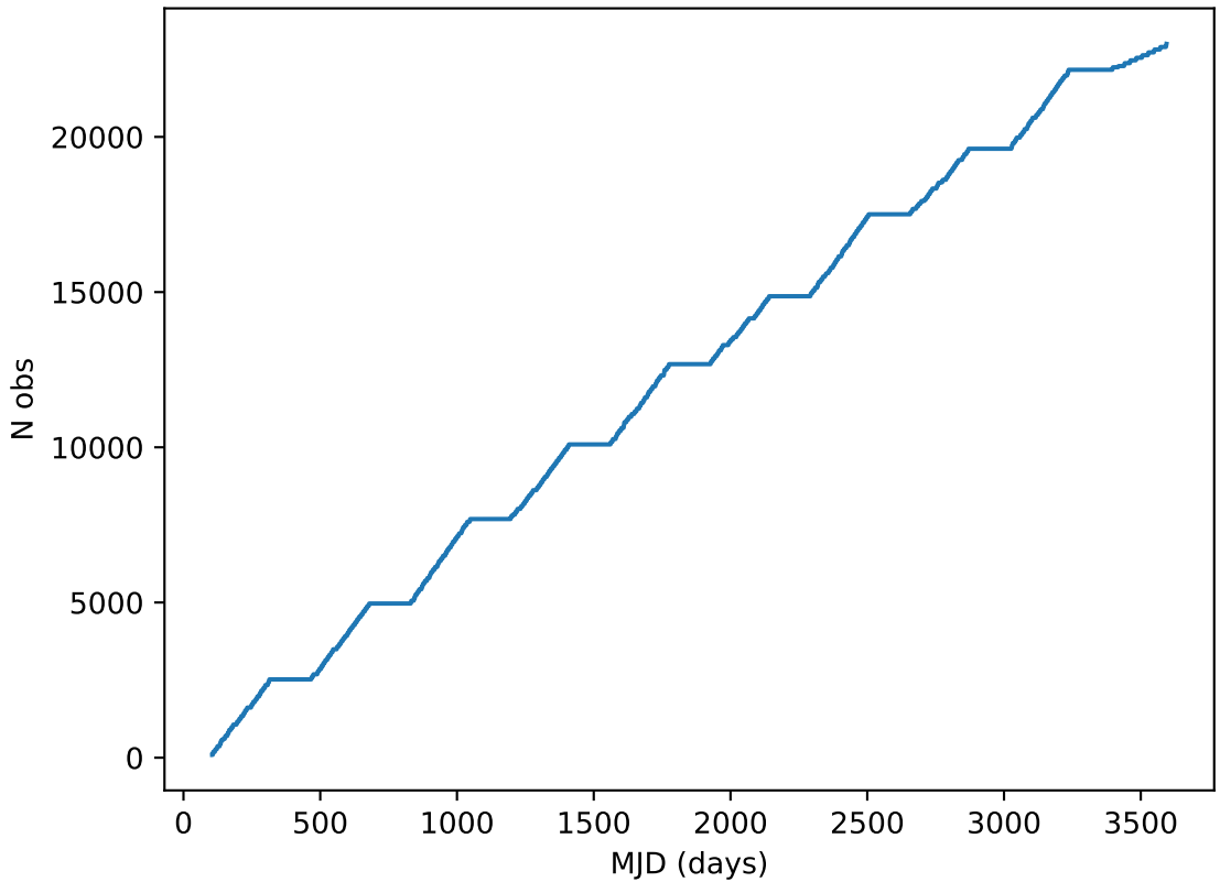
internal_u_expt60_nscale1.2v3.4_10yrs all bands: DD:EDFS Cumulative NVisits
