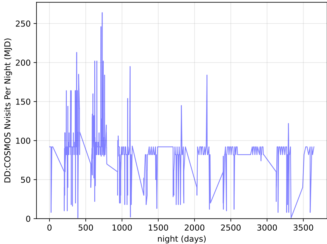
internal_u_expt60_nscale1.2v3.4_10yrs all bands: DD: COSMOS Nvisits Per Night
