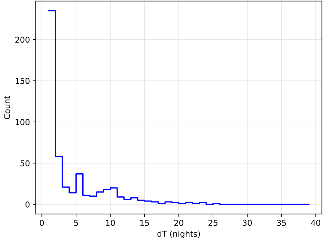
internal_u_expt60_nscale1.2v3.4_10yrs all bands: DD: COSMOS Delta Nights Histogram
