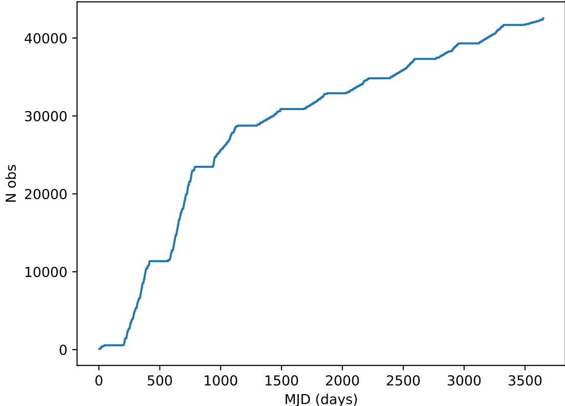
internal_u_expt60_nscale1.2v3.4_10yrs all bands: DD: COSMOS Cumulative NVisits
