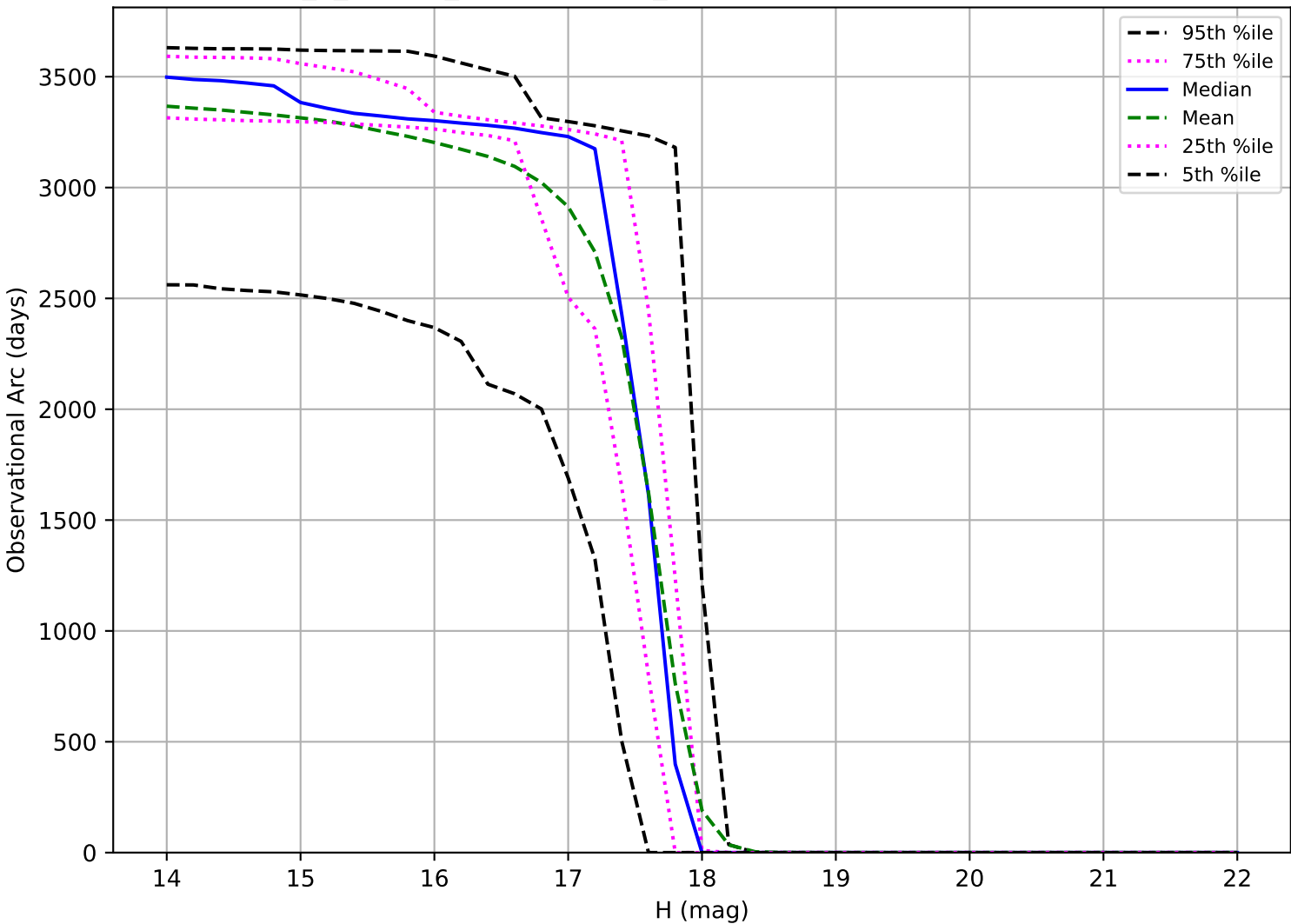
internal_u_expt60_nscale1.1v3.4_10yrs: Observational Arc Length Trojan
