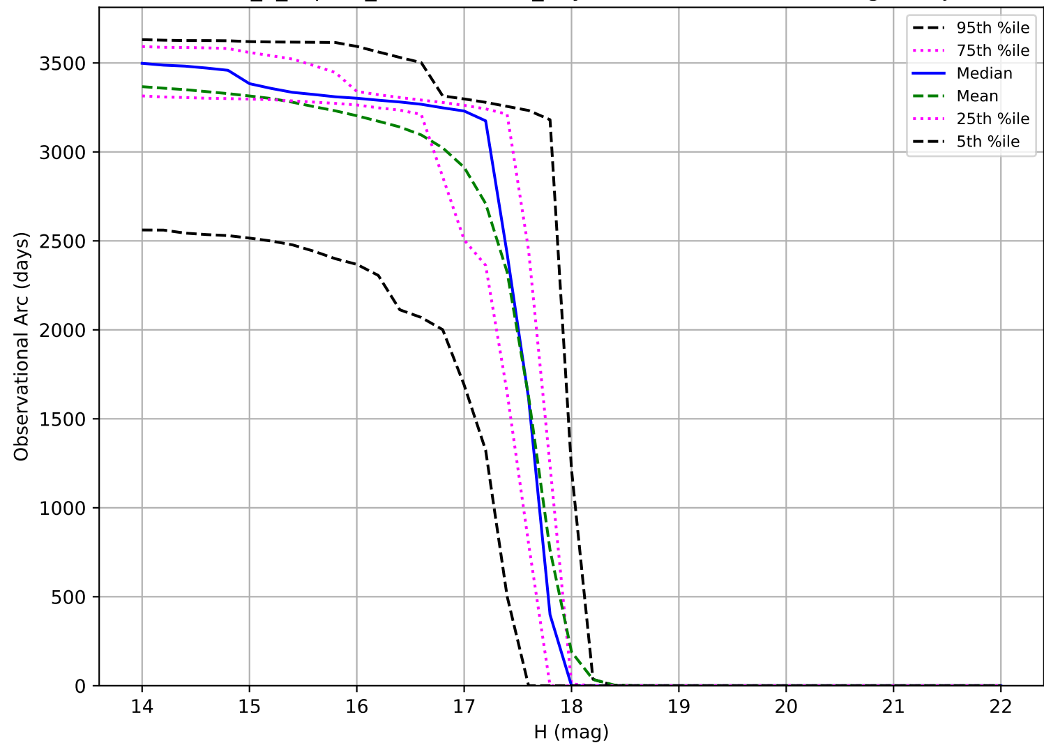
internal_u_expt60_nscale1.1v3.4_10yrs: Observational Arc Length Trojan
