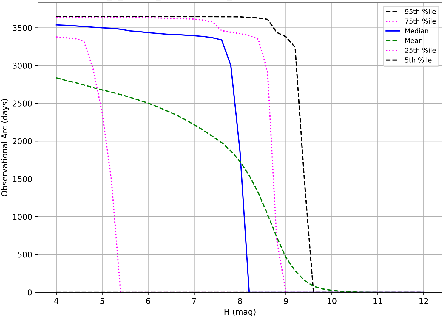
internal_u_expt60_nscale1.1v3.4_10yrs: Observational Arc Length TNO
