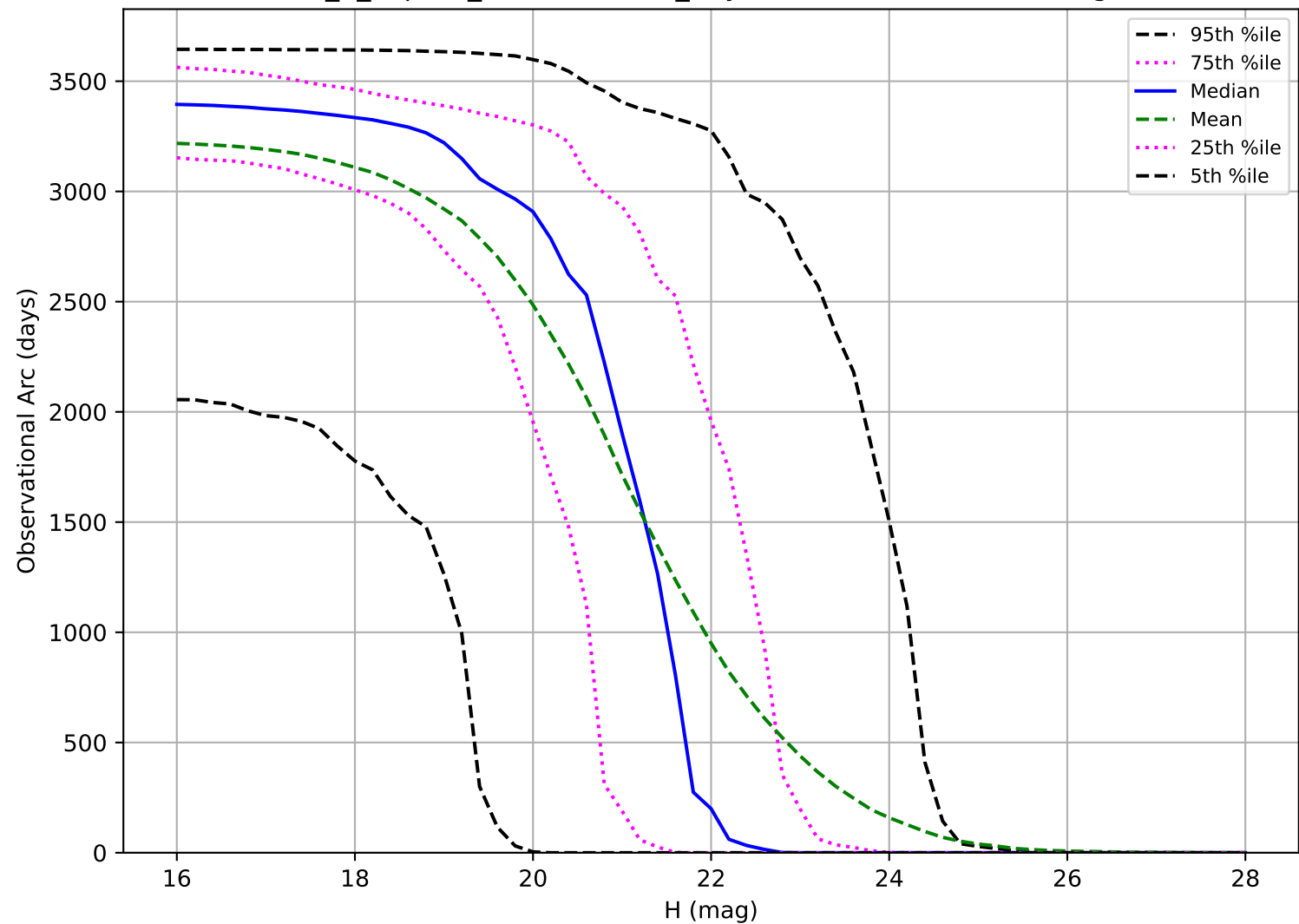
internal_u_expt60_nscale1.1v3.4_10yrs: Observational Arc Length PHA
