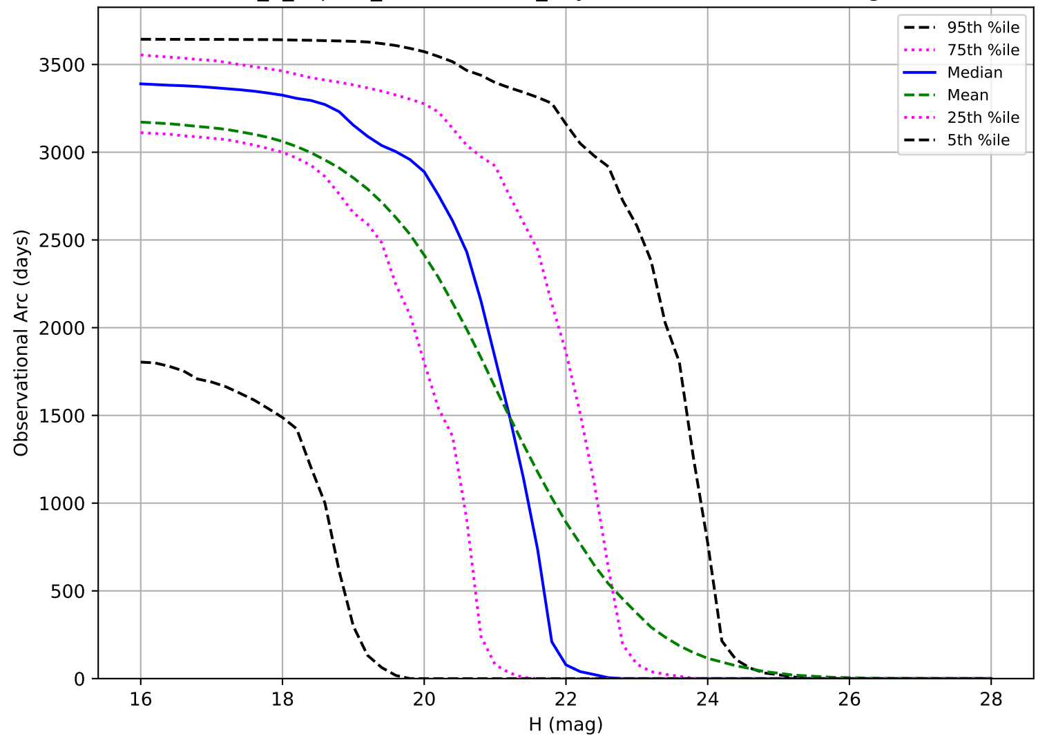
internal_u_expt60_nscale1.1v3.4_10yrs: Observational Arc Length NEO
