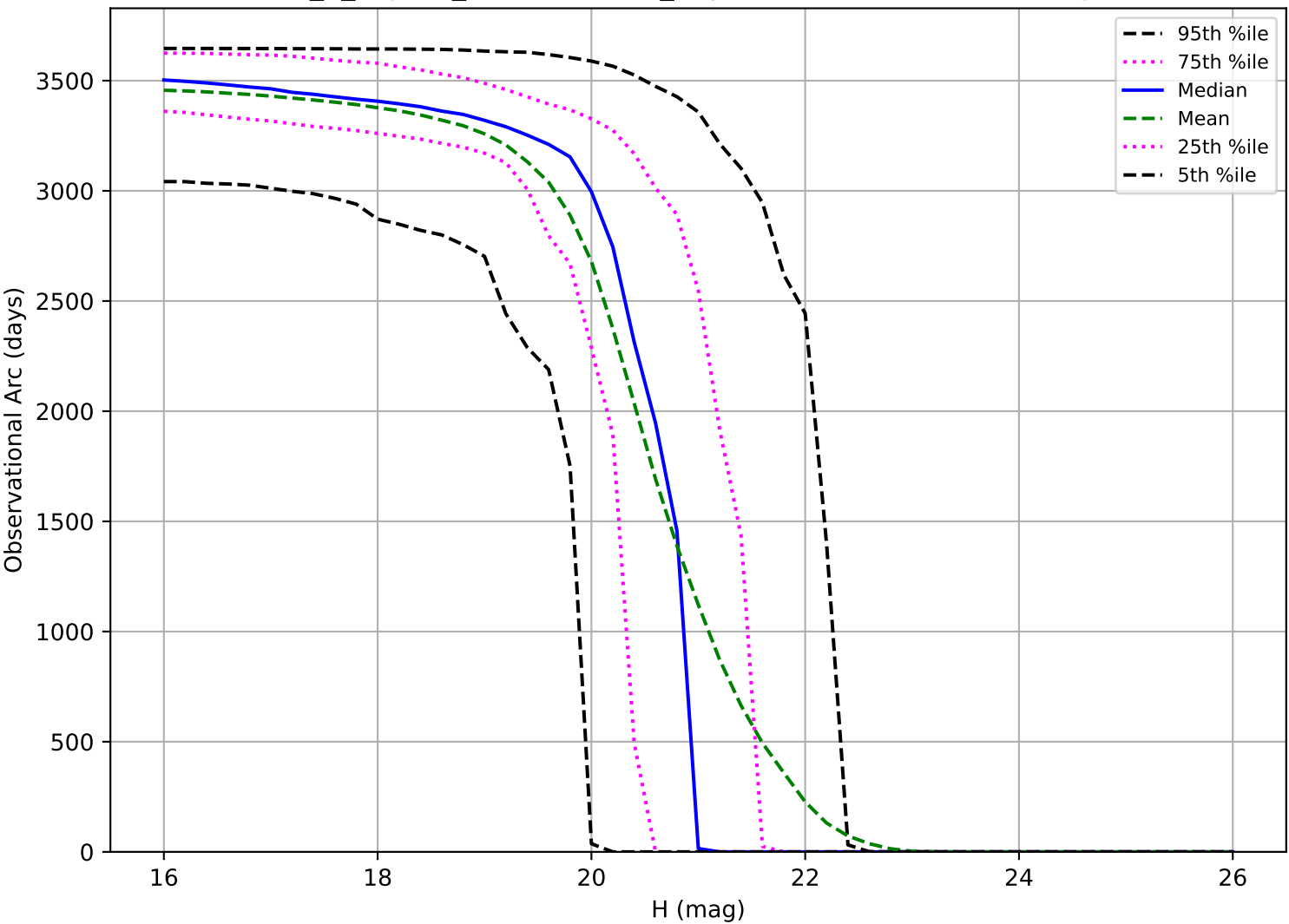
internal_u_expt60_nscale1.1v3.4_10yrs: Observational Arc Length MBA
