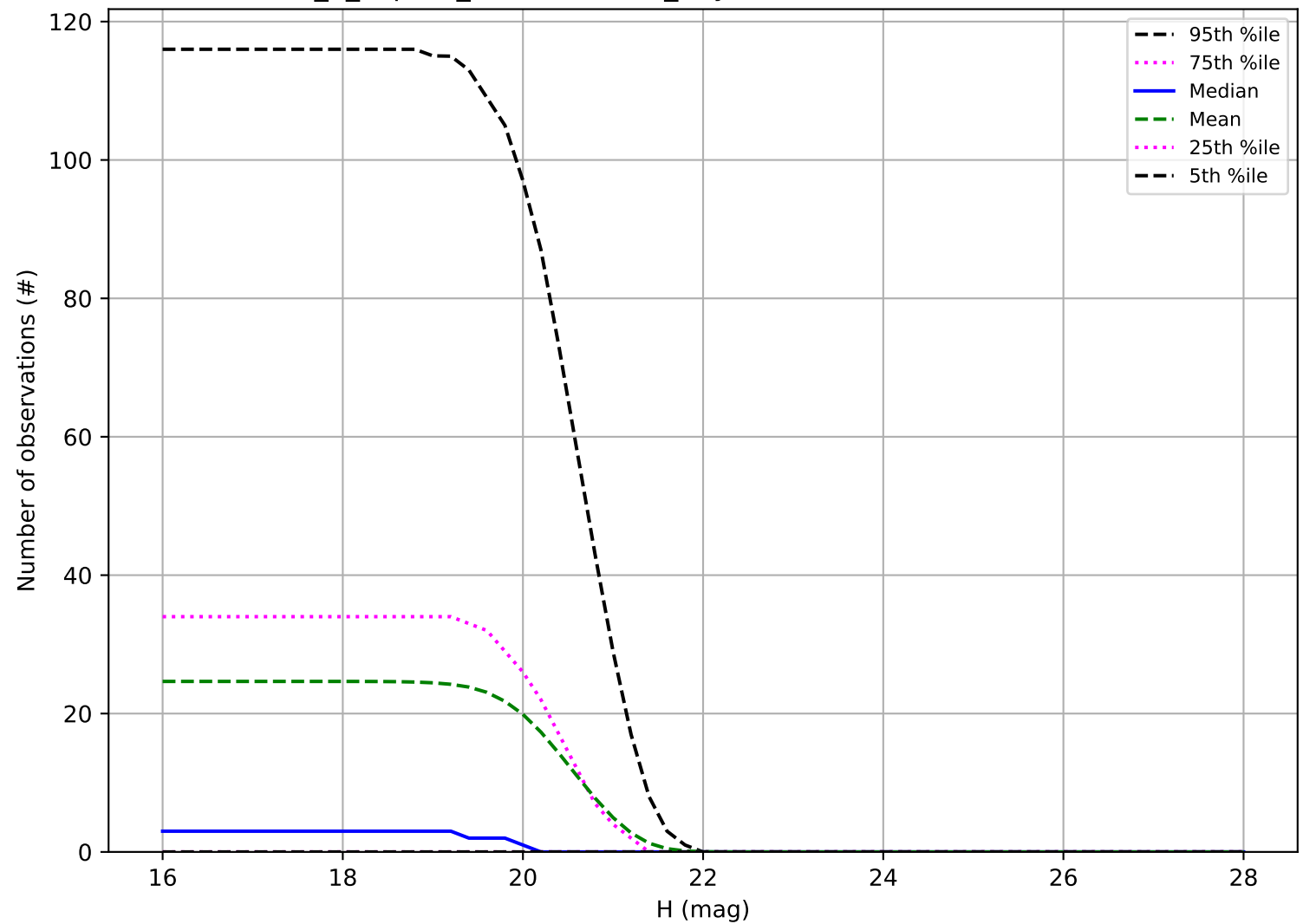
internal_u_expt60_nscale1.1v3.4_10yrs: Number of observations Vatira
