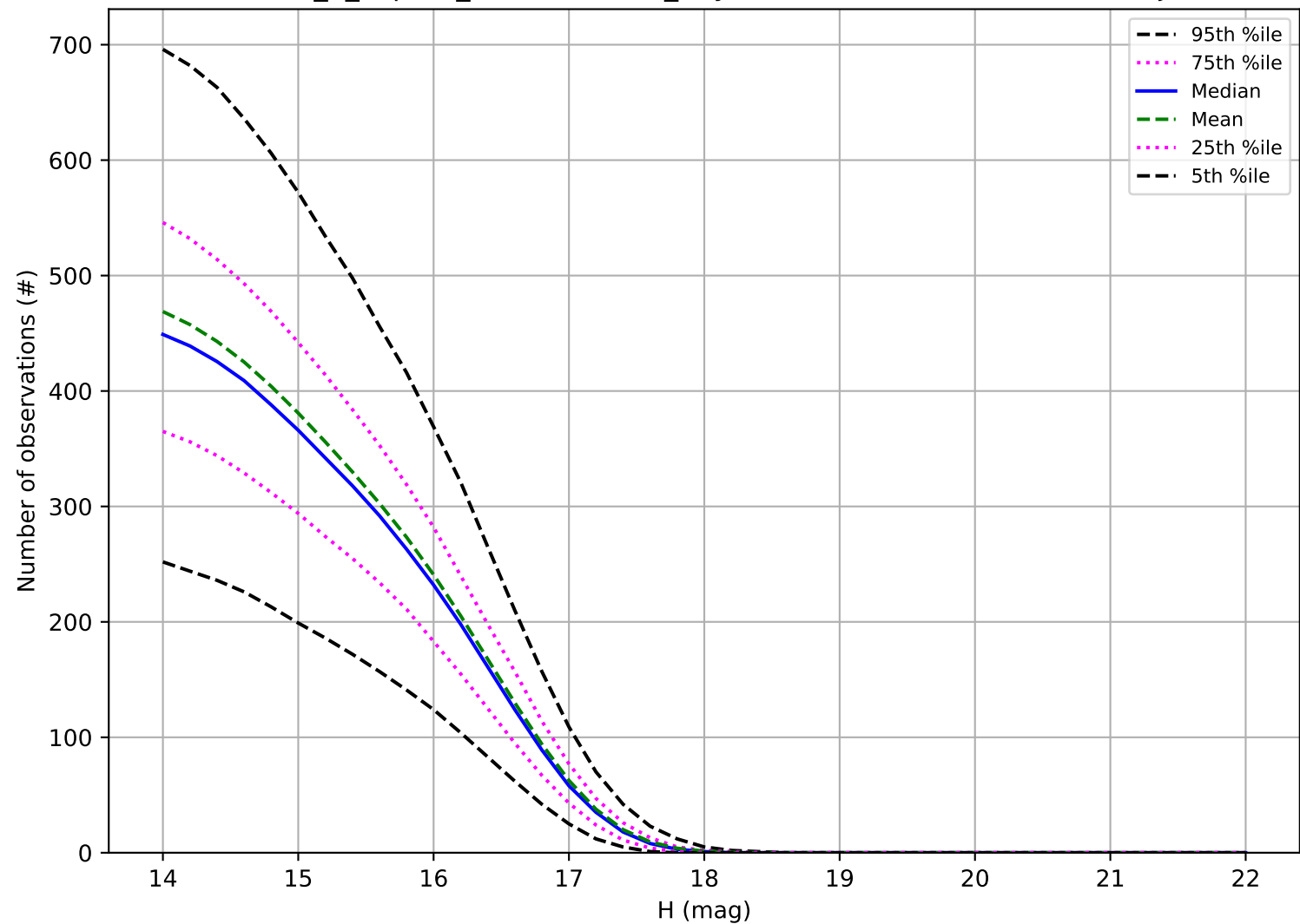
internal_u_expt60_nscale1.1v3.4_10yrs: Number of observations Trojan
