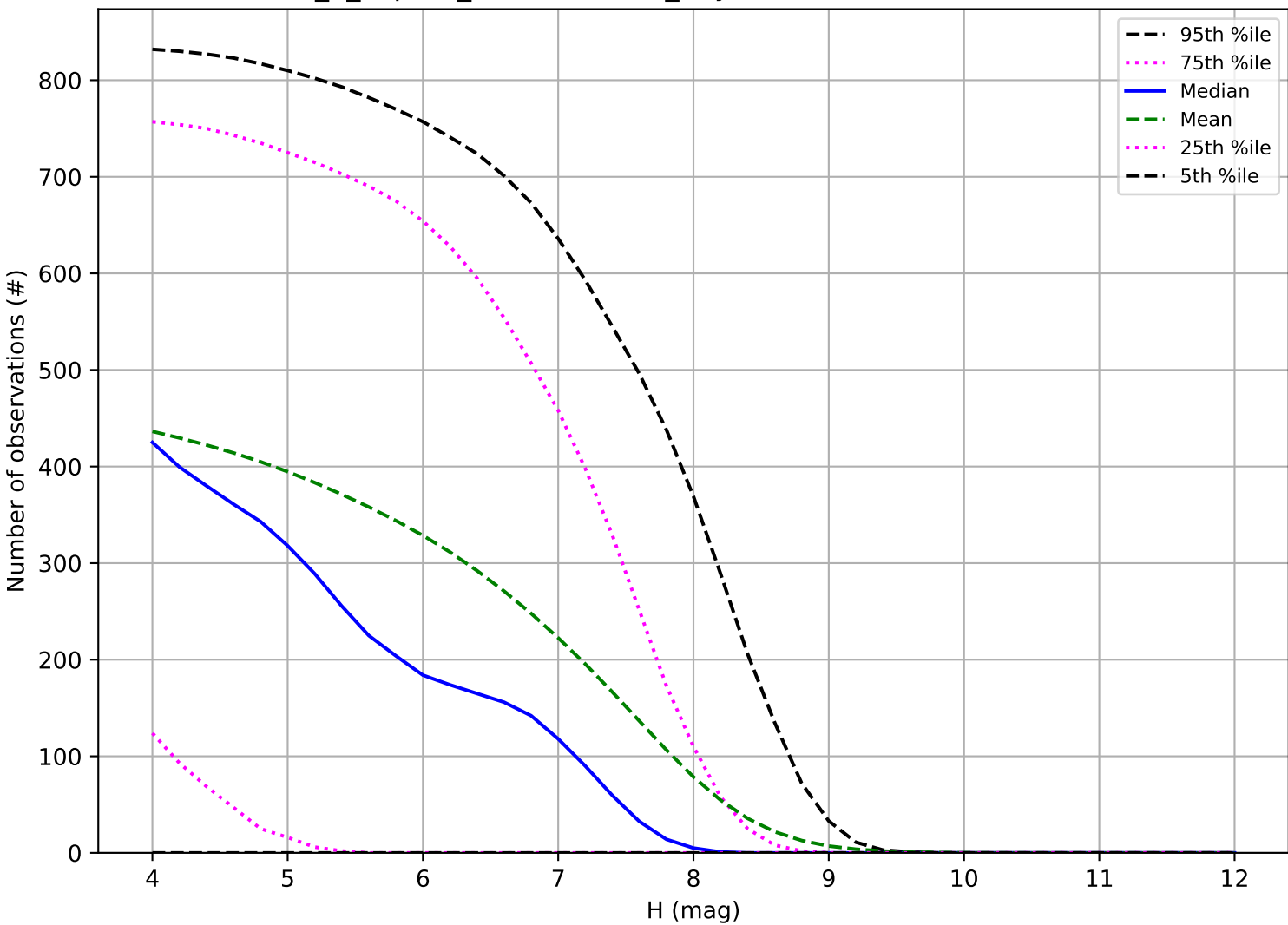
internal_u_expt60_nscale1.1v3.4_10yrs: Number of observations TNO
