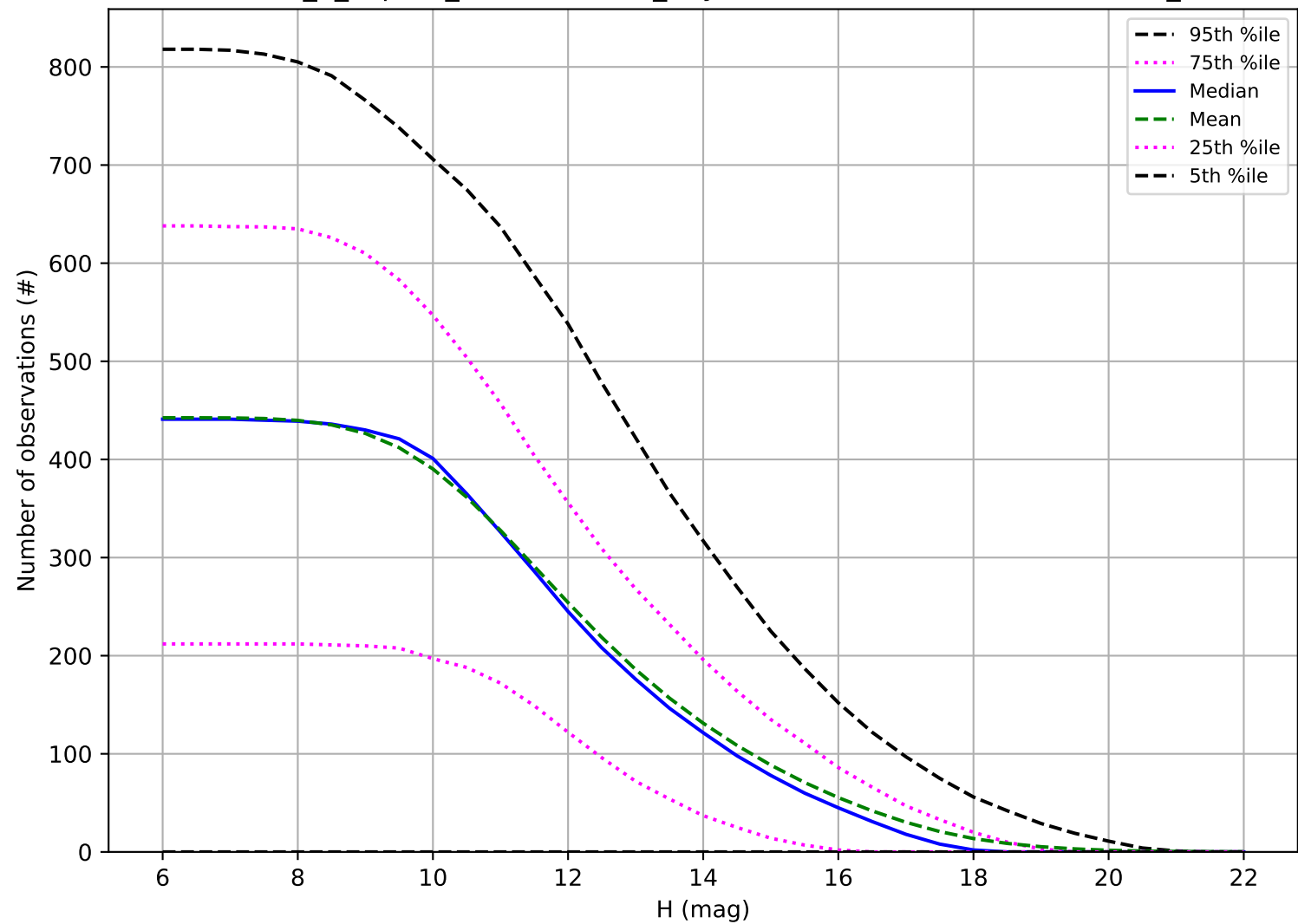
internal_u_expt60_nscale1.1v3.4_10yrs: Number of observations OCC_r5
