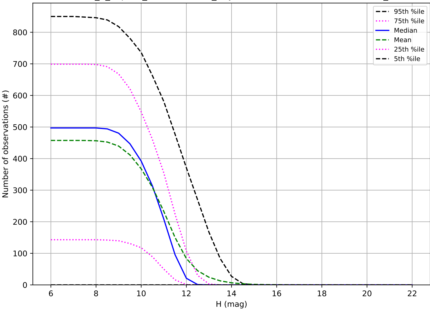
internal_u_expt60_nscale1.1v3.4_10yrs: Number of observations OCC_r20
