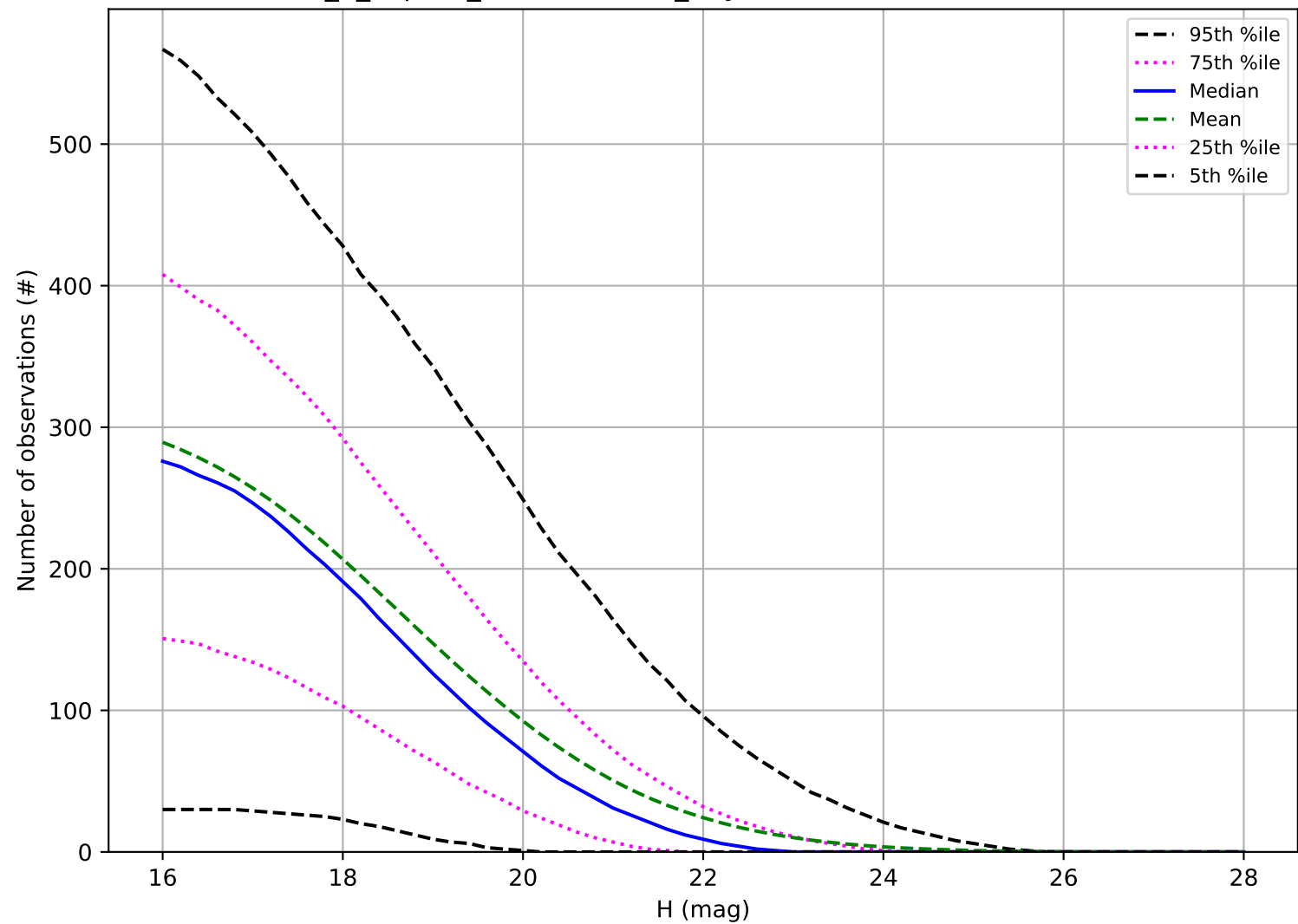
internal_u_expt60_nscale1.1v3.4_10yrs: Number of observations NEO
