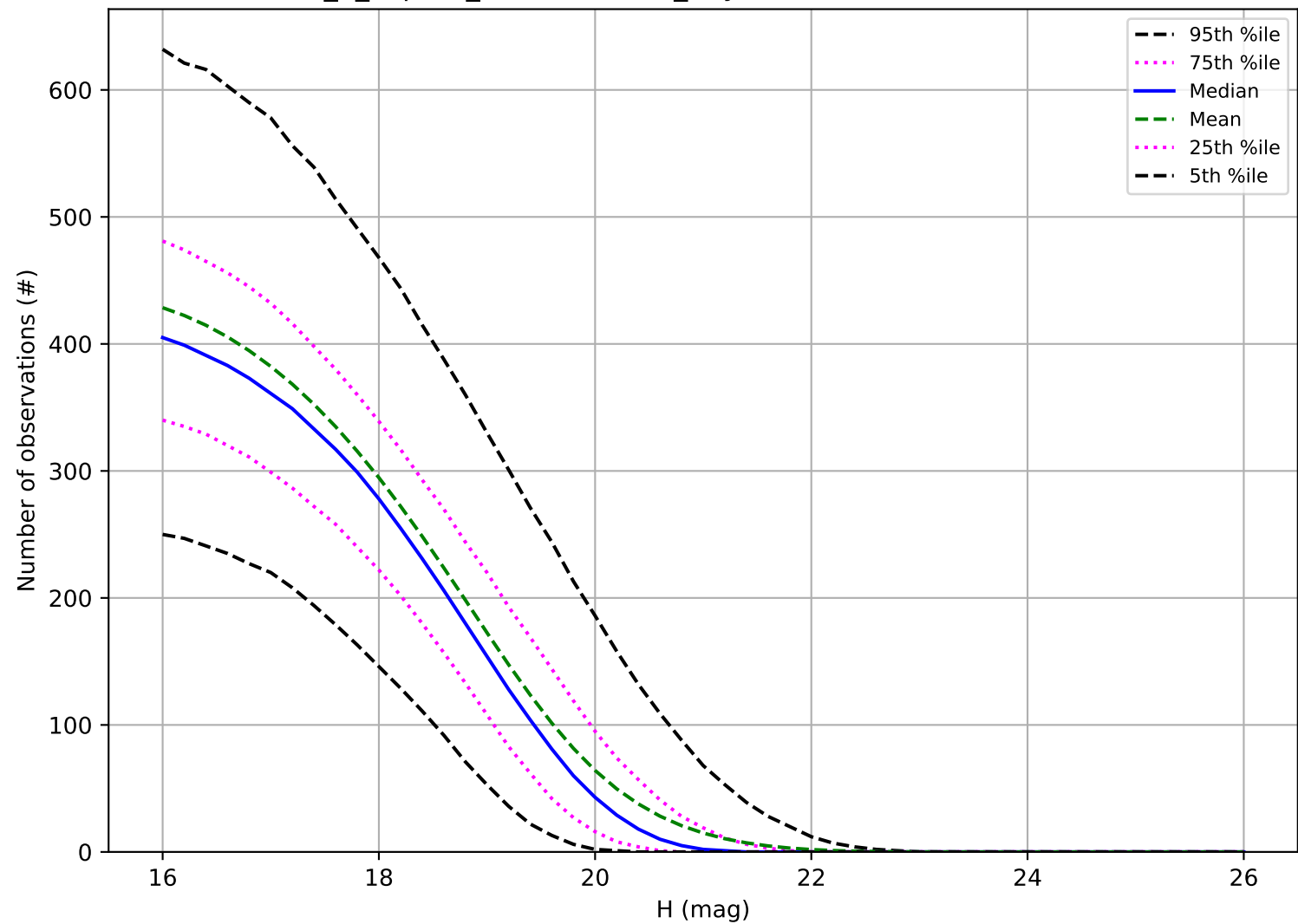
internal_u_expt60_nscale1.1v3.4_10yrs: Number of observations MBA
