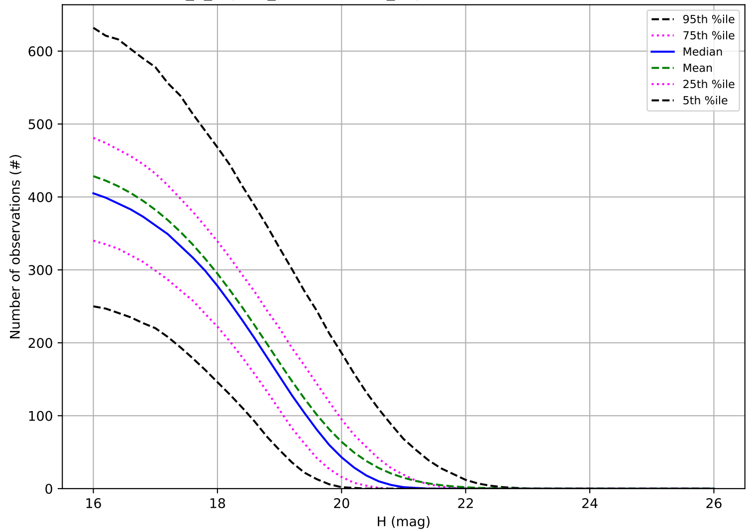
internal_u_expt60_nscale1.1v3.4_10yrs: Number of observations MBA
