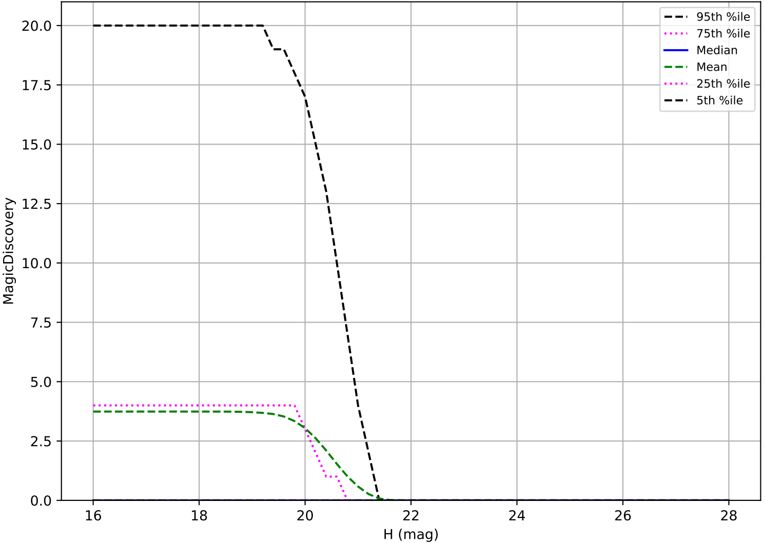
internal_u_expt60_nscale1.1v3.4_10yrs: Vatira 6 detections in 60 nights detection loss
