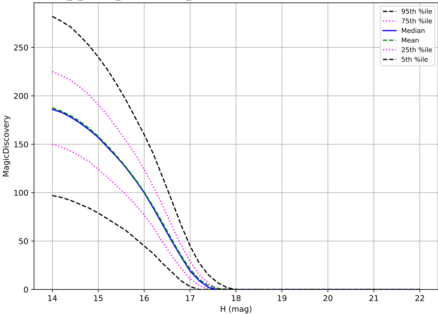
internal_u_expt60_nscale1.1v3.4_10yrs: Trojan 6 detections in 60 nights detection loss
