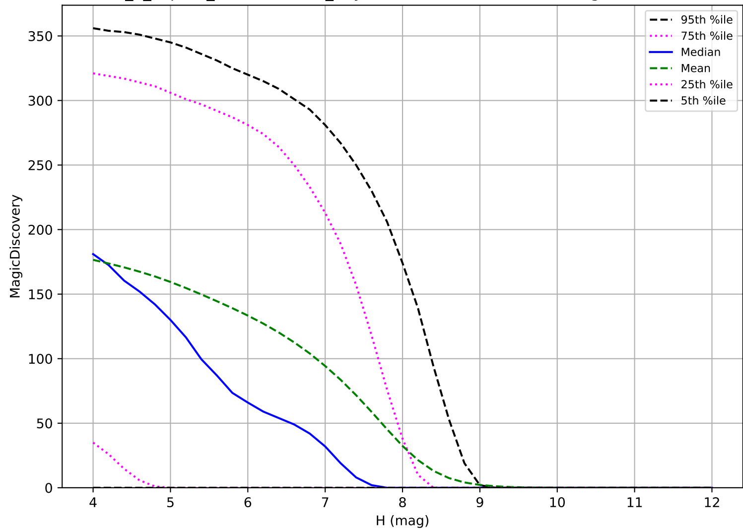
internal_u_expt60_nscale1.1v3.4_10yrs: TNO 6 detections in 60 nights detection loss
