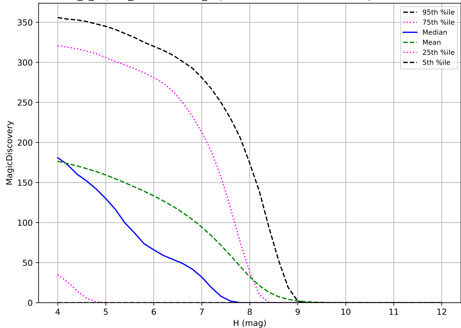
internal_u_expt60_nscale1.1v3.4_10yrs: TNO 6 detections in 60 nights detection loss
