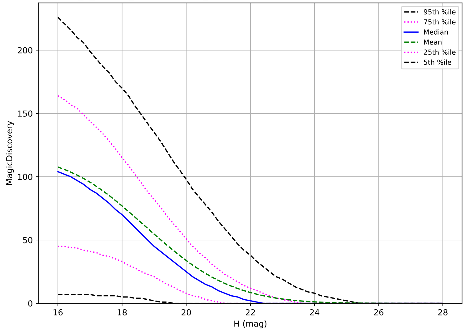
internal_u_expt60_nscale1.1v3.4_10yrs: PHA 6 detections in 60 nights detection loss
