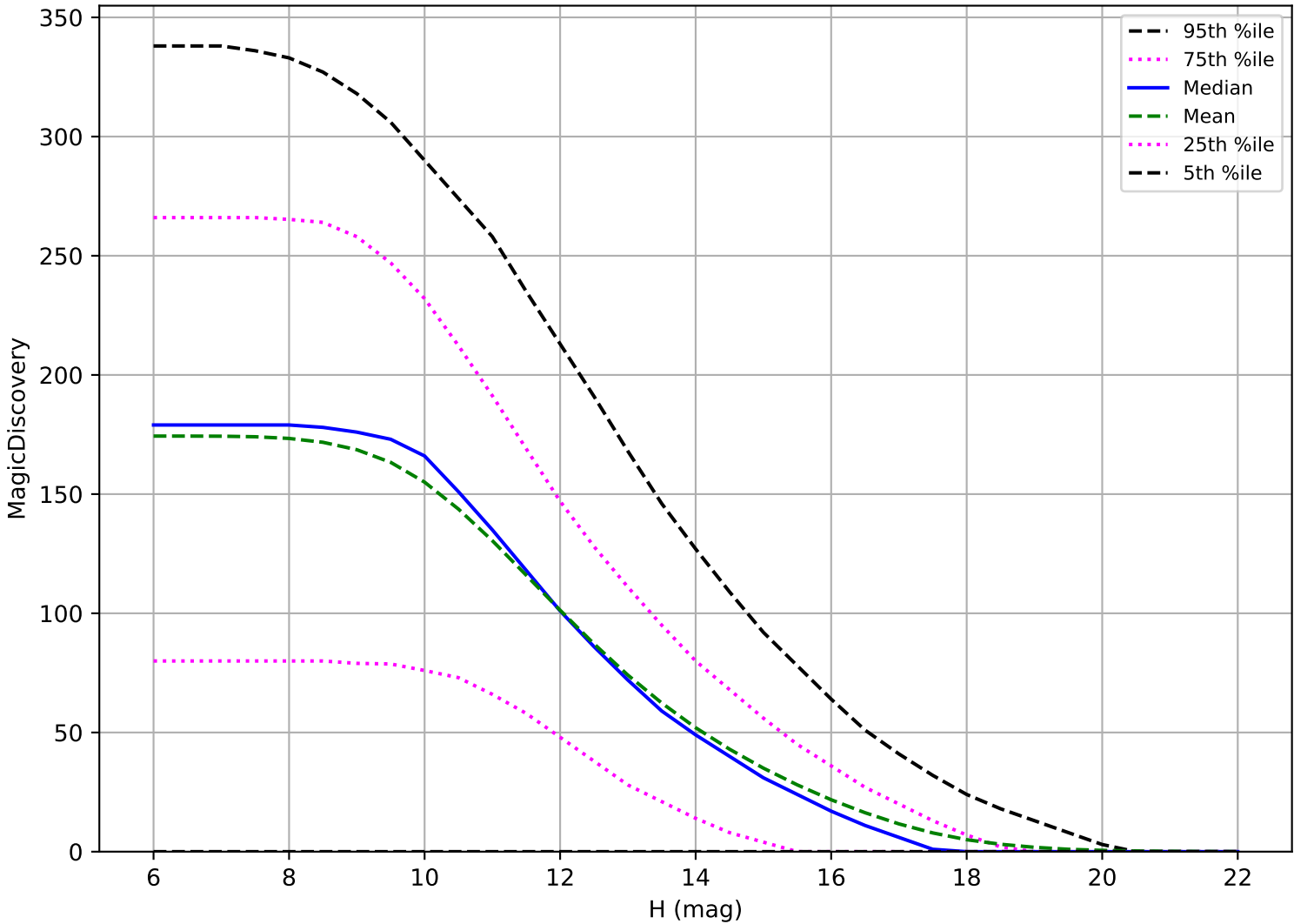
internal_u_expt60_nscale1.1v3.4_10yrs: OCC_r5 6 detections in 60 nights detection loss
