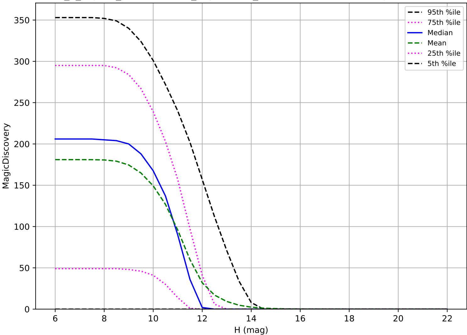
internal_u_expt60_nscale1.1v3.4_10yrs: OCC_r20 6 detections in 60 nights detection loss
