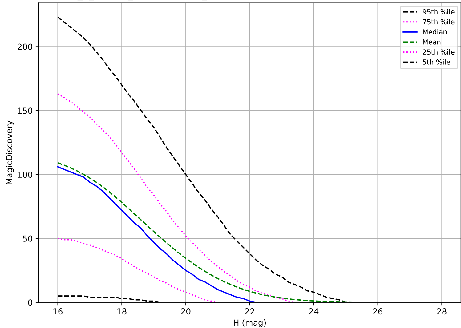
internal_u_expt60_nscale1.1v3.4_10yrs: NEO 6 detections in 60 nights detection loss
