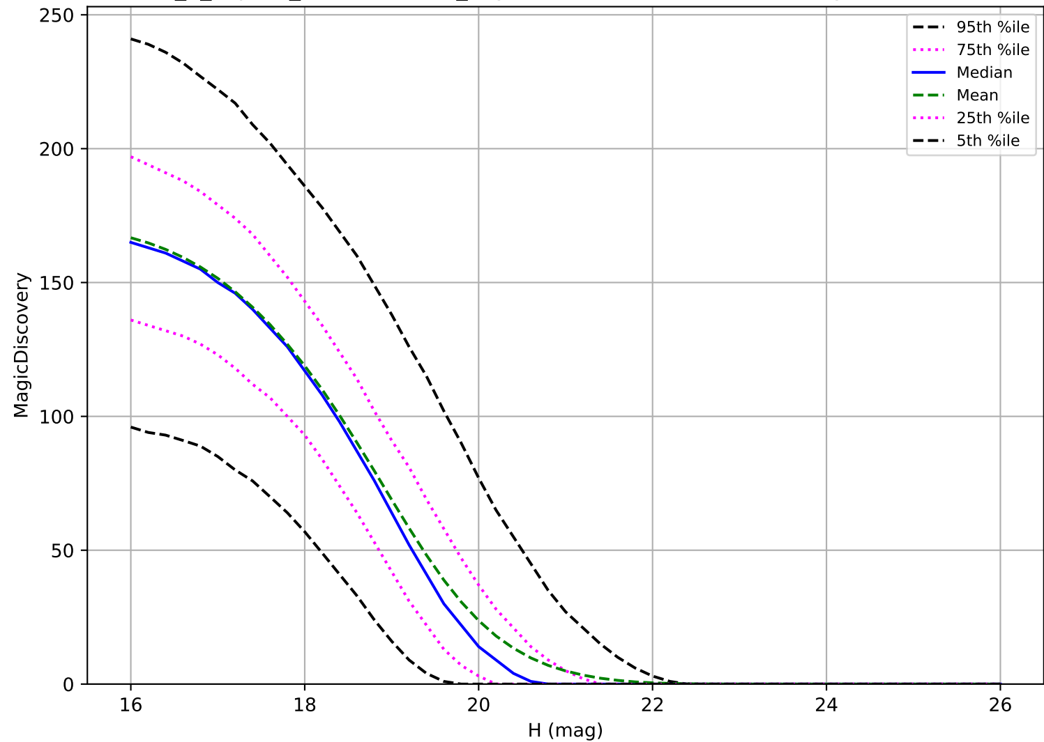
internal_u_expt60_nscale1.1v3.4_10yrs: MBA 6 detections in 60 nights detection loss
