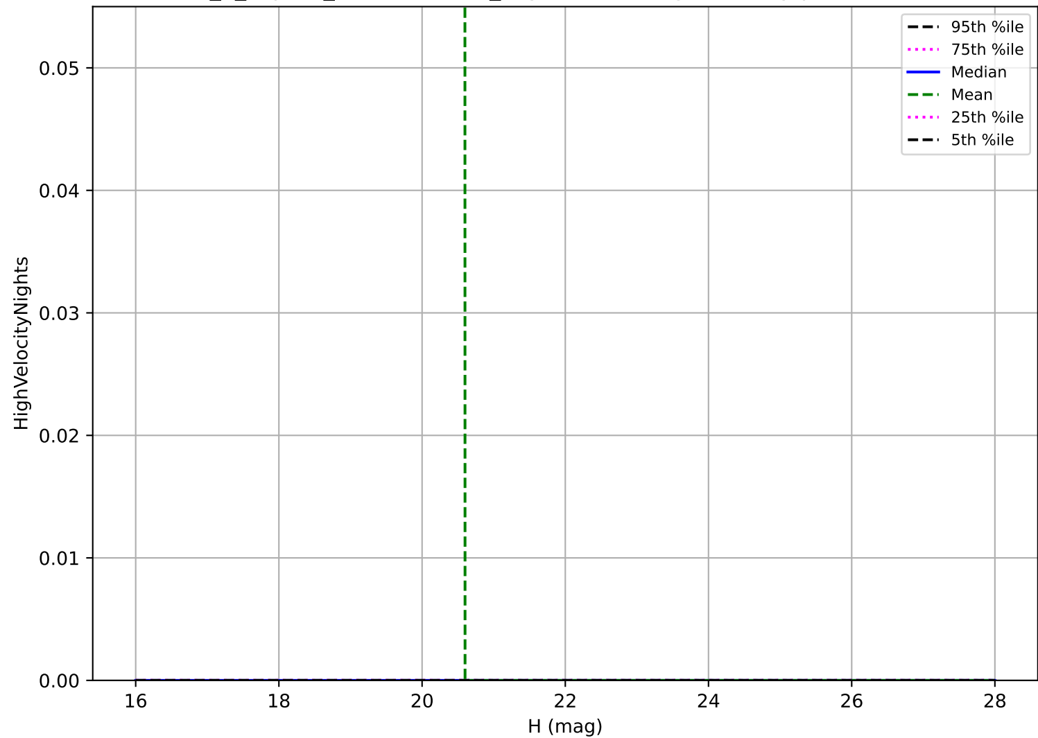
internal_u_expt60_nscale1.1v3.4_10yrs: Vatira High velocity pair detection loss
