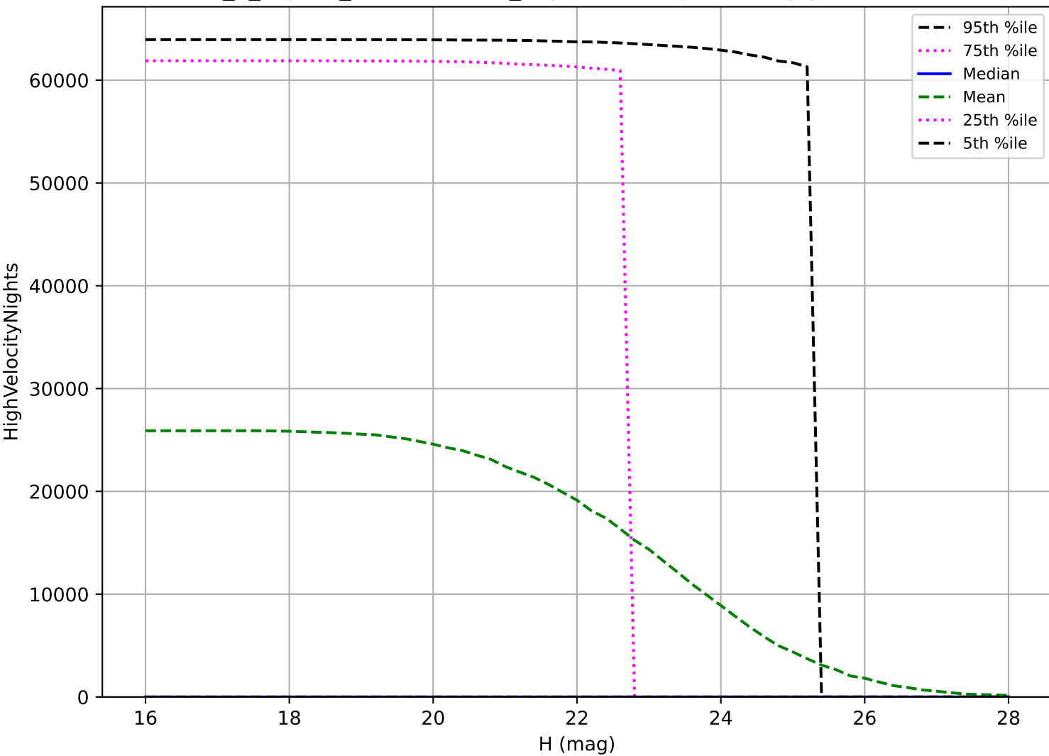
internal_u_expt60_nscale1.1v3.4_10yrs: PHA High velocity pair detection loss
