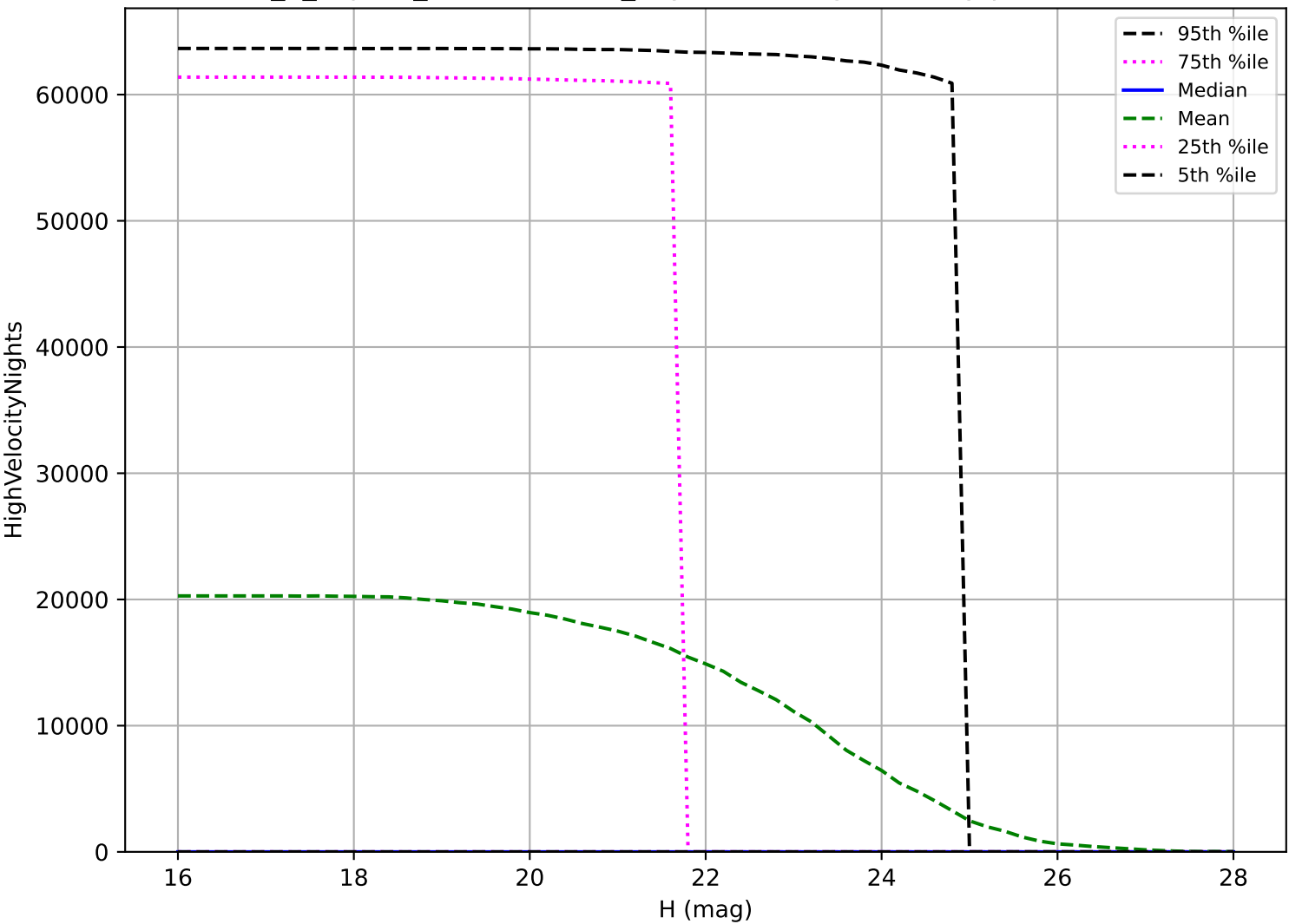
internal_u_expt60_nscale1.1v3.4_10yrs: NEO High velocity pair detection loss
