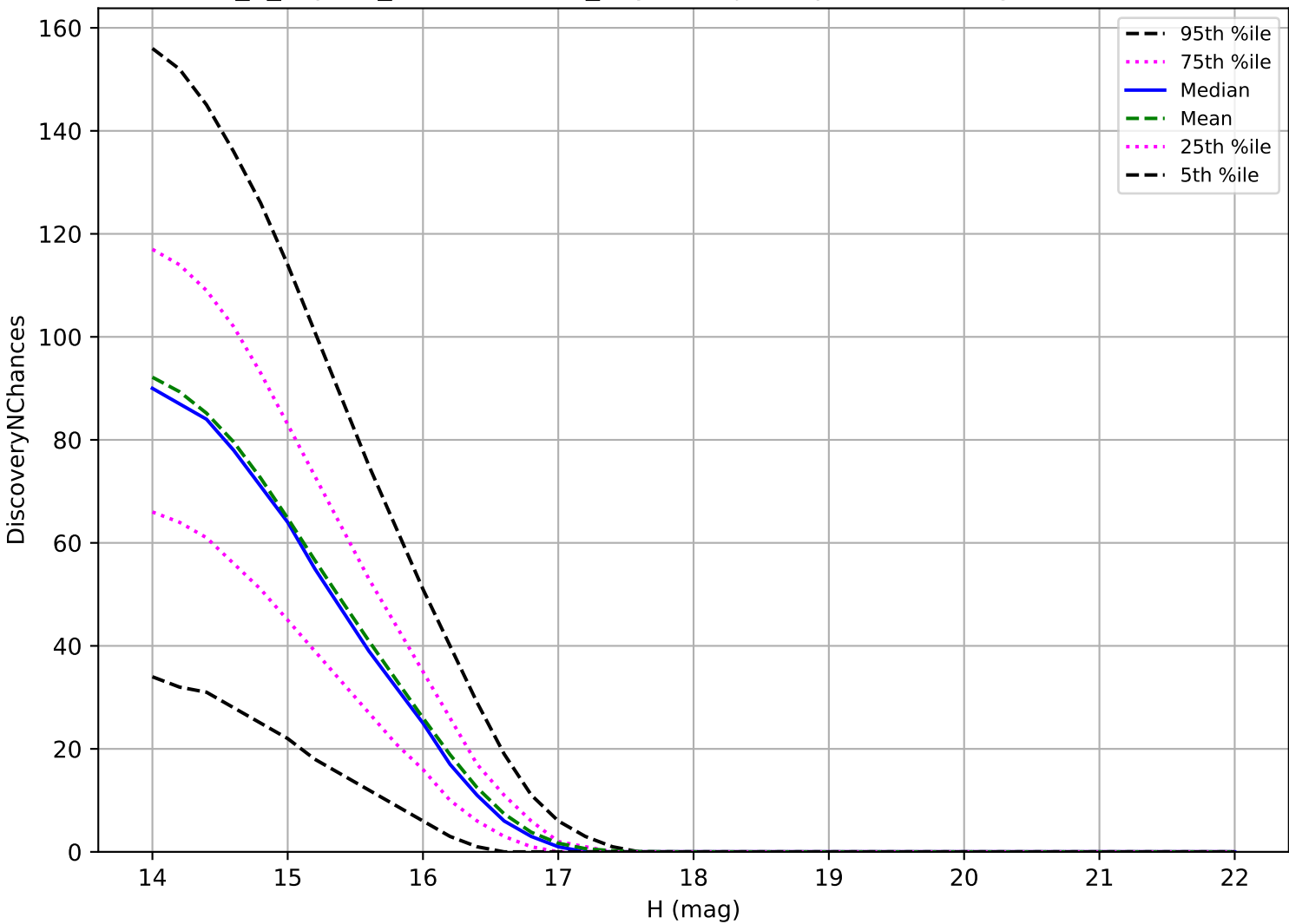
internal_u_expt60_nscale1.1v3.4_10yrs: Trojan 3 pairs in 15 nights detection loss
