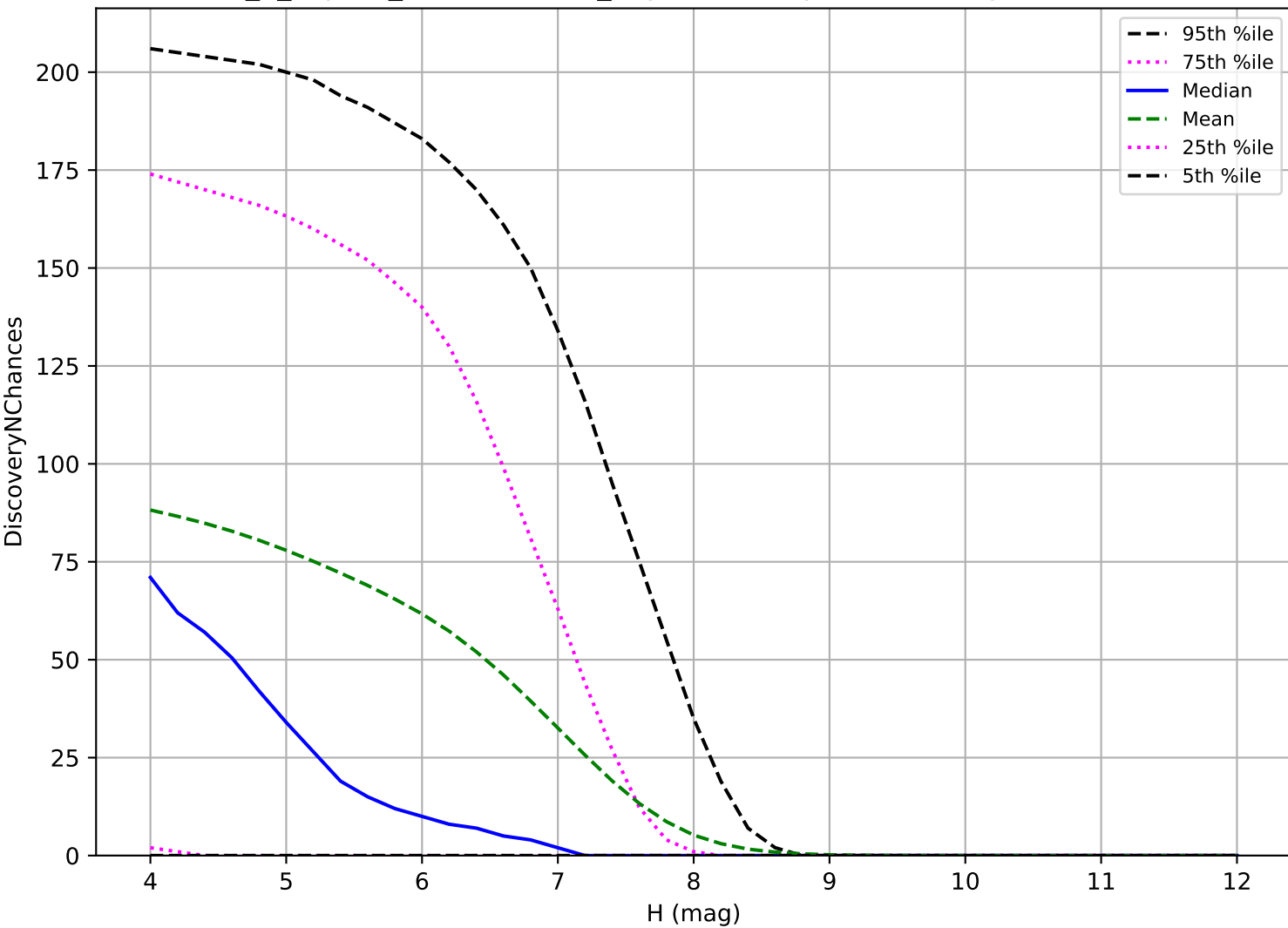
internal_u_expt60_nscale1.1v3.4_10yrs: TNO 3 pairs in 15 nights detection loss
