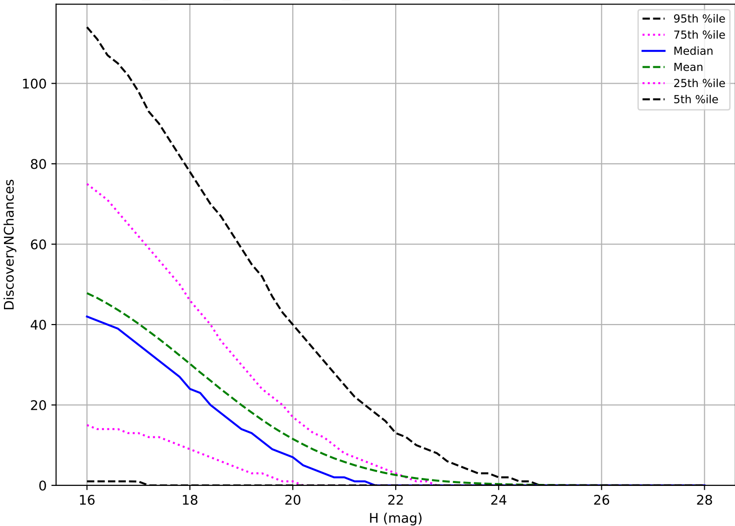
internal_u_expt60_nscale1.1v3.4_10yrs: PHA 3 pairs in 15 nights detection loss
