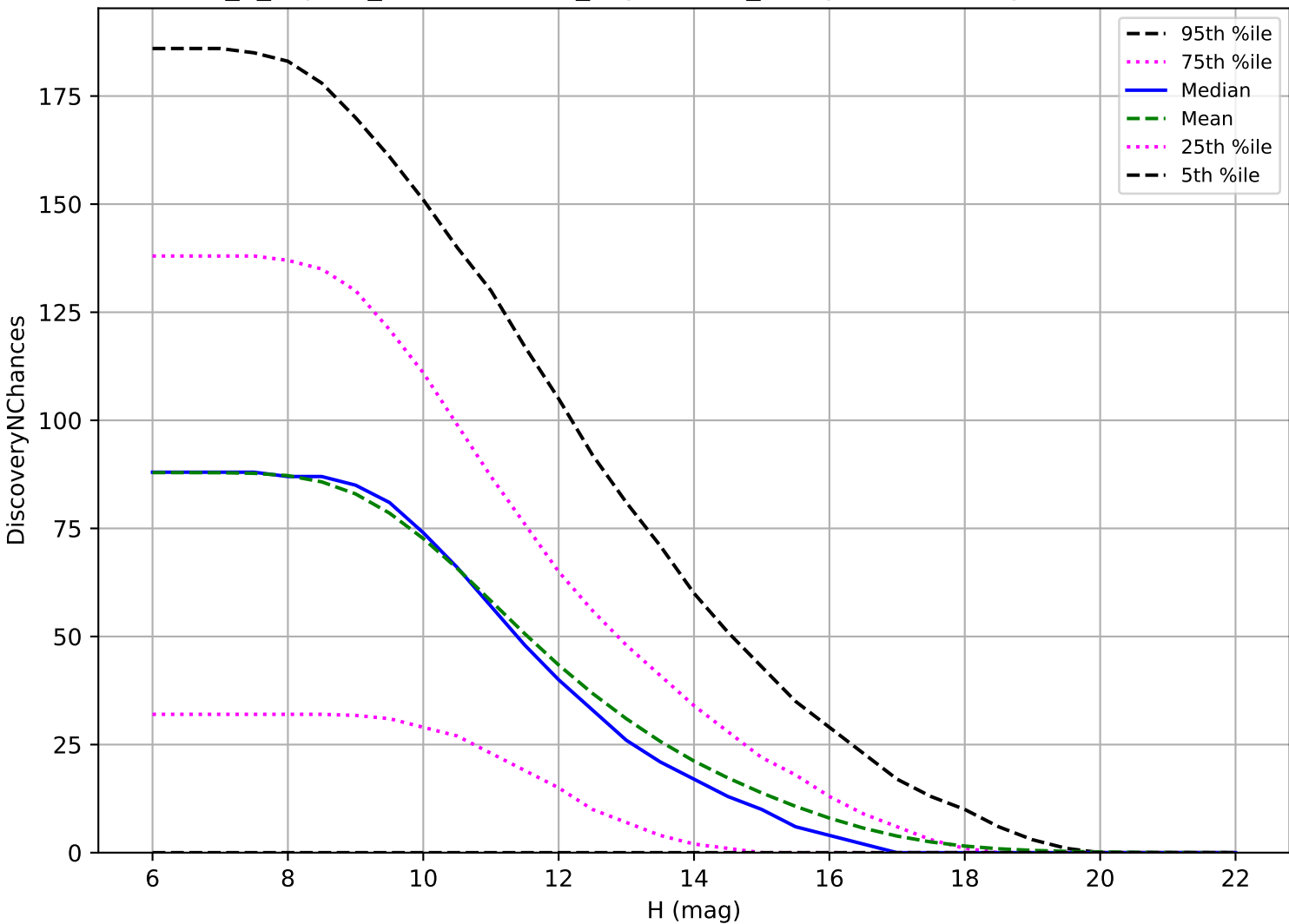
internal_u_expt60_nscale1.1v3.4_10yrs: OCC_r5 3 pairs in 15 nights detection loss
