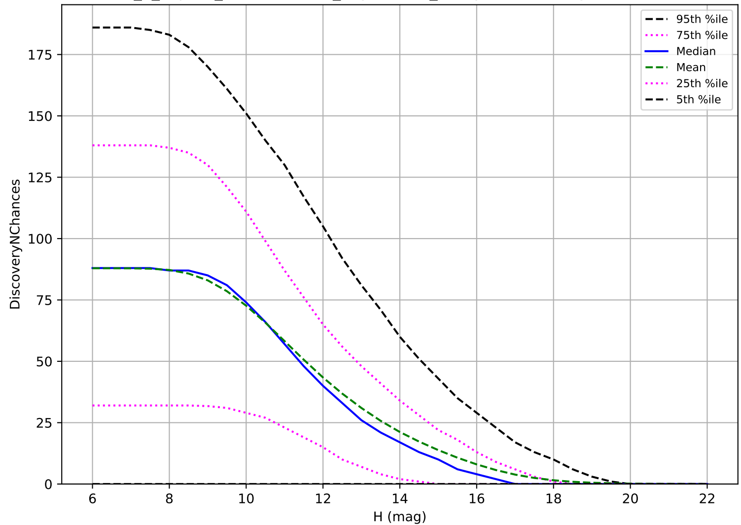
internal_u_expt60_nscale1.1v3.4_10yrs: OCC_r5 3 pairs in 15 nights detection loss
