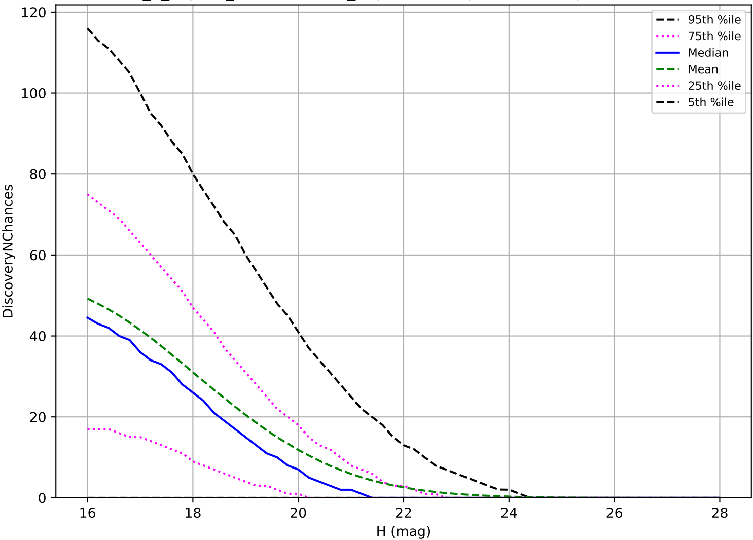
internal_u_expt60_nscale1.1v3.4_10yrs: NEO 3 pairs in 15 nights detection loss
