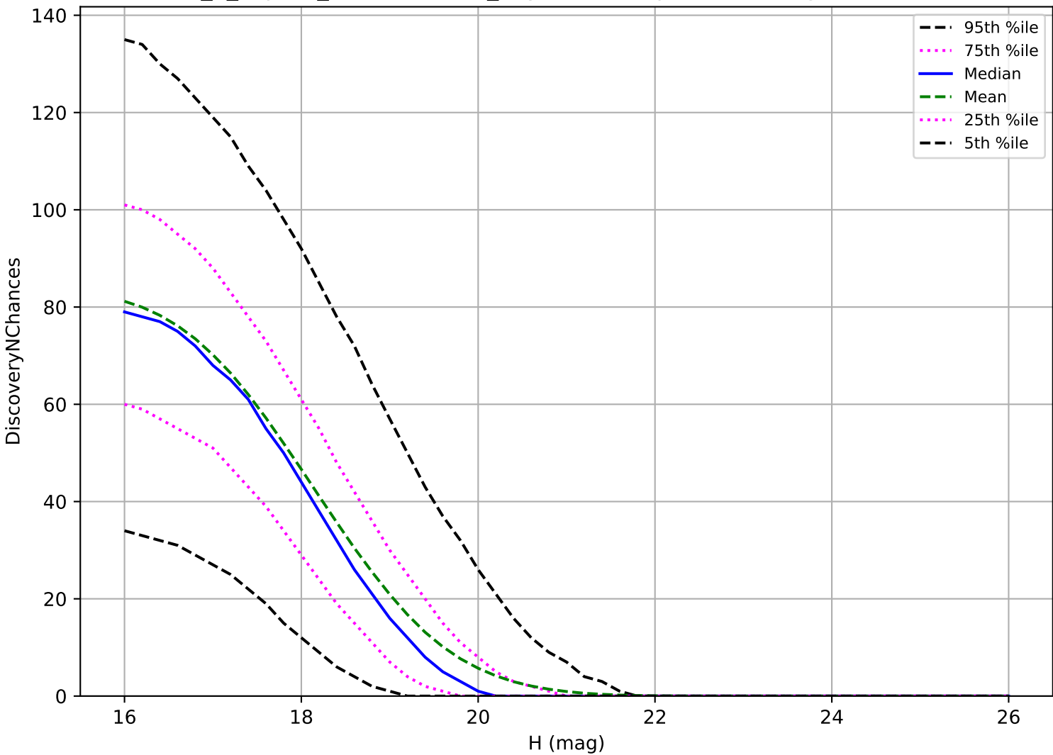
internal_u_expt60_nscale1.1v3.4_10yrs: MBA 3 pairs in 15 nights detection loss
