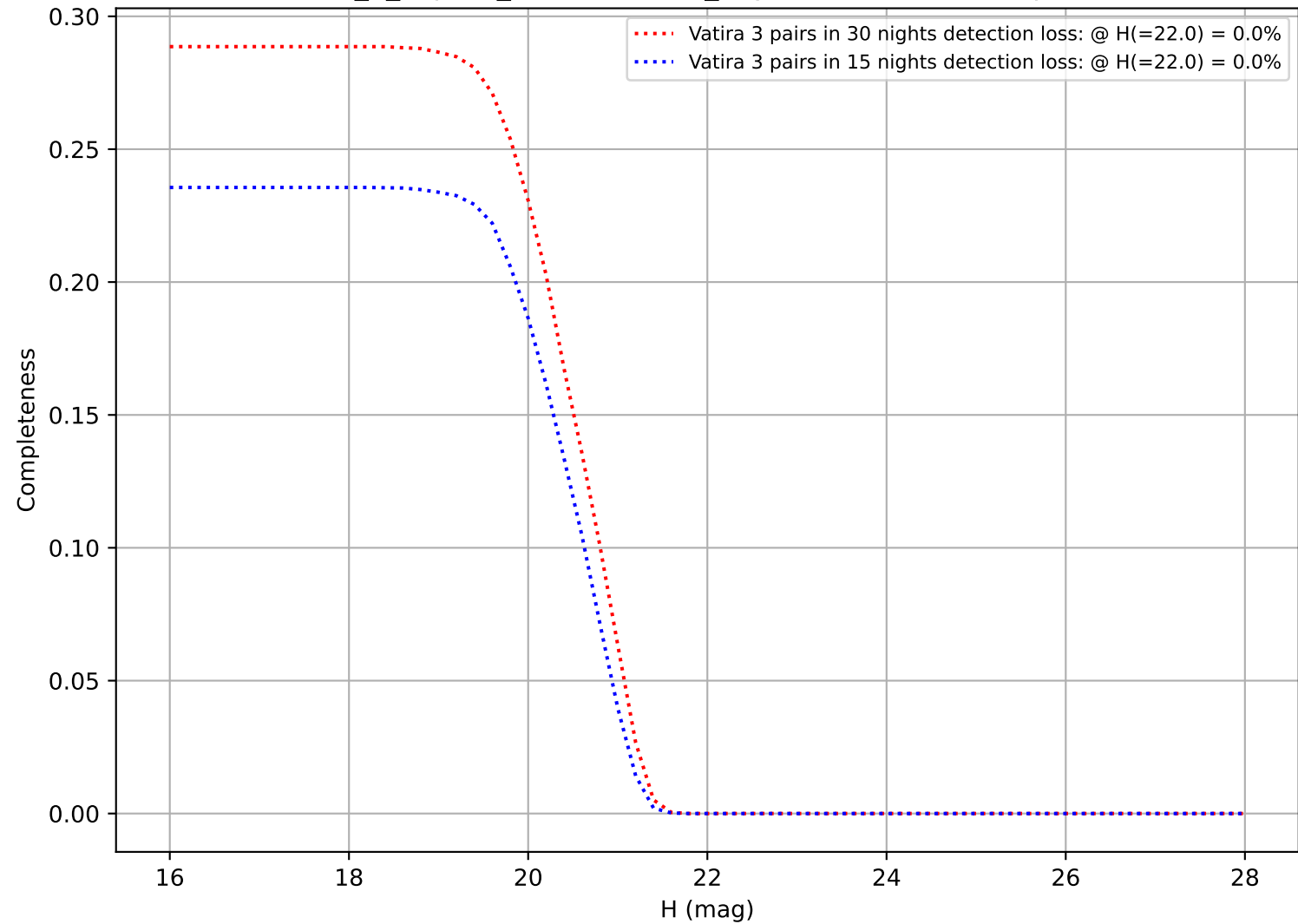
internal_u_expt60_nscale1.1v3.4_10yrs: DifferentialCompleteness
