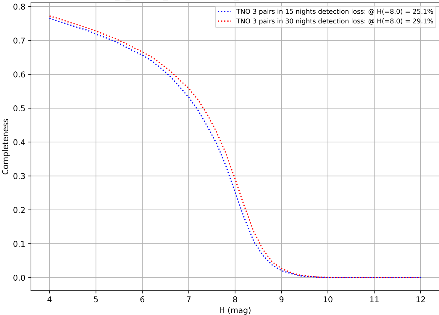
internal_u_expt60_nscale1.1v3.4_10yrs: DifferentialCompleteness
