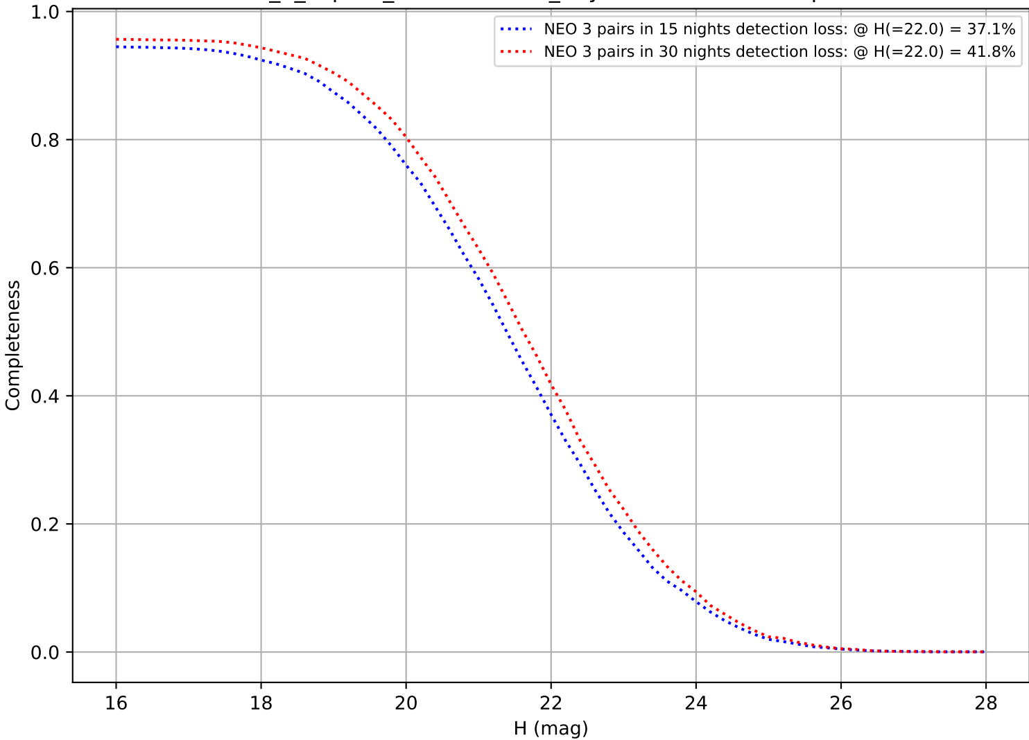
internal_u_expt60_nscale1.1v3.4_10yrs: DifferentialCompleteness
