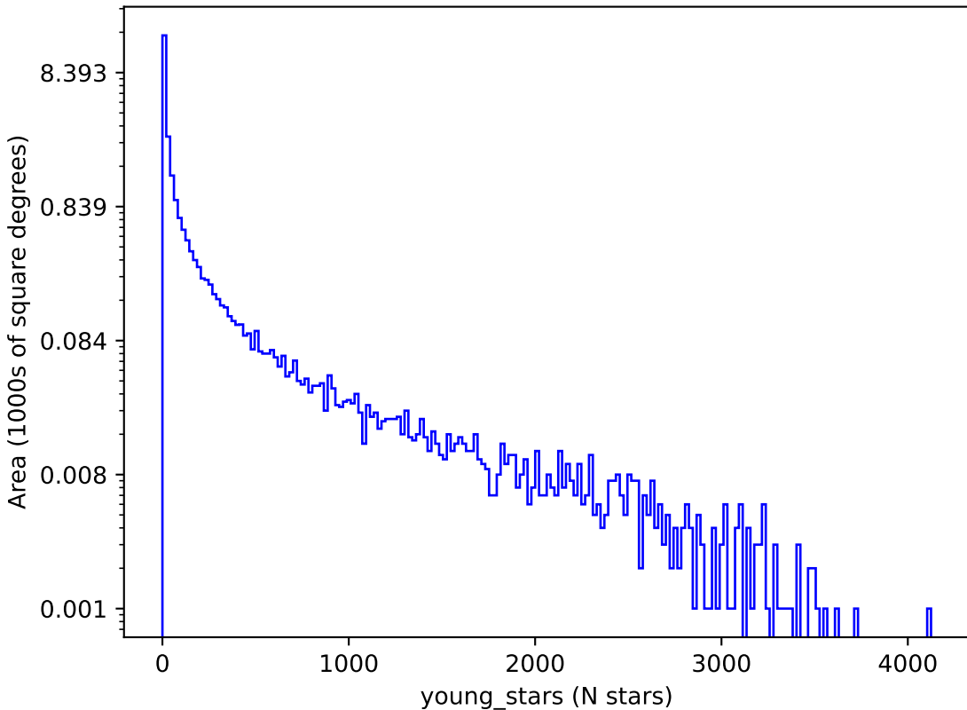
internal_u_expt60_nscale1.1v3.4_10yrs : young_stars
