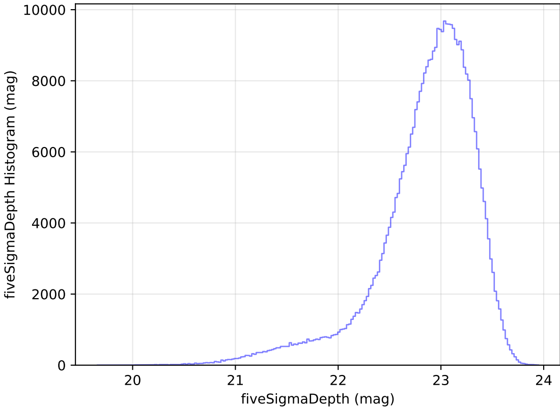
internal_u_expt60_nscale1.1v3.4_10yrs z: fiveSigmaDepth Histogram
