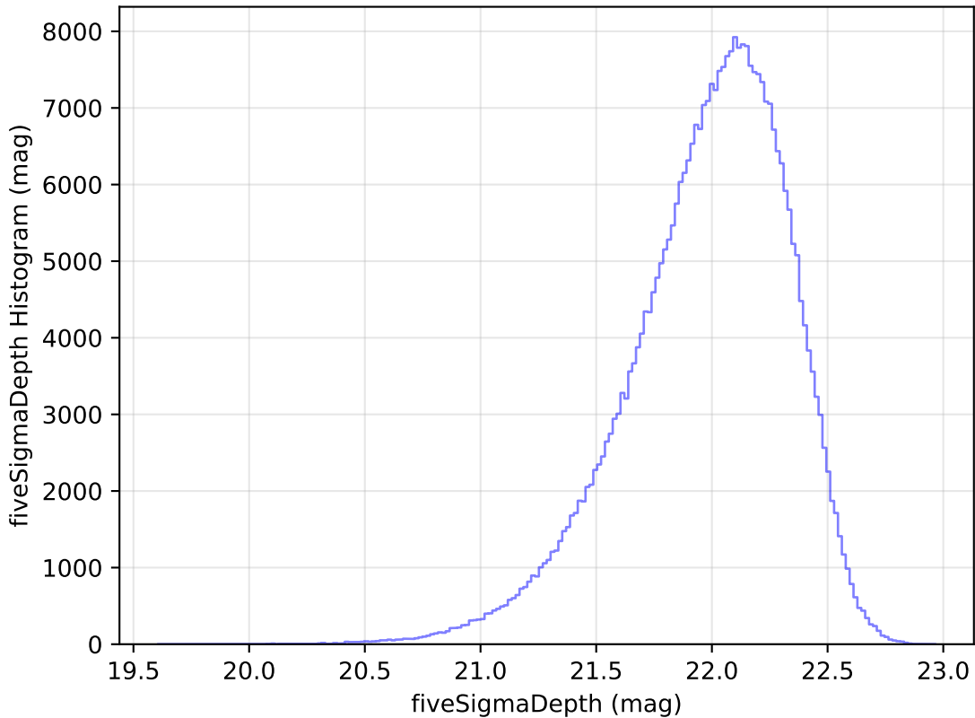
internal_u_expt60_nscale1.1v3.4_10yrs y: fiveSigmaDepth Histogram
