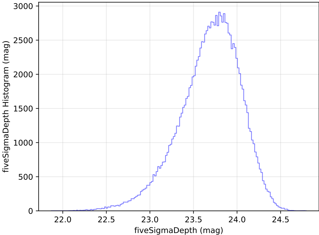
internal_u_expt60_nscale1.1v3.4_10yrs u: fiveSigmaDepth Histogram
