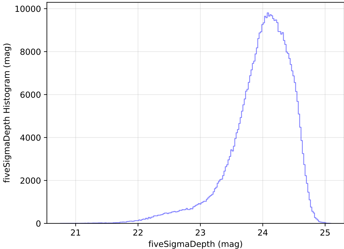
internal_u_expt60_nscale1.1v3.4_10yrs r: fiveSigmaDepth Histogram
