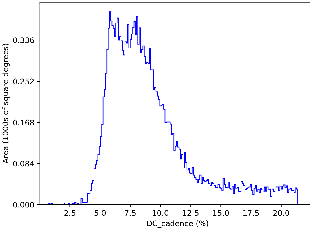
internal_u_expt60_nscale1.1v3.4_10yrs : TDC_cadence
