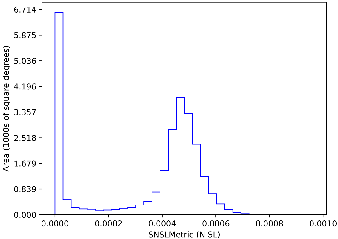
internal_u_expt60_nscale1.1v3.4_10yrs : SNSLMetric
