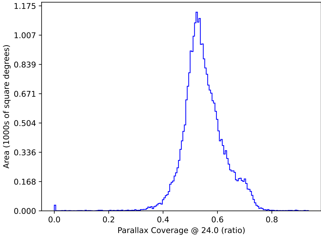
internal_u_expt60_nscale1.1v3.4_10yrs : Parallax Coverage @ 24.0
