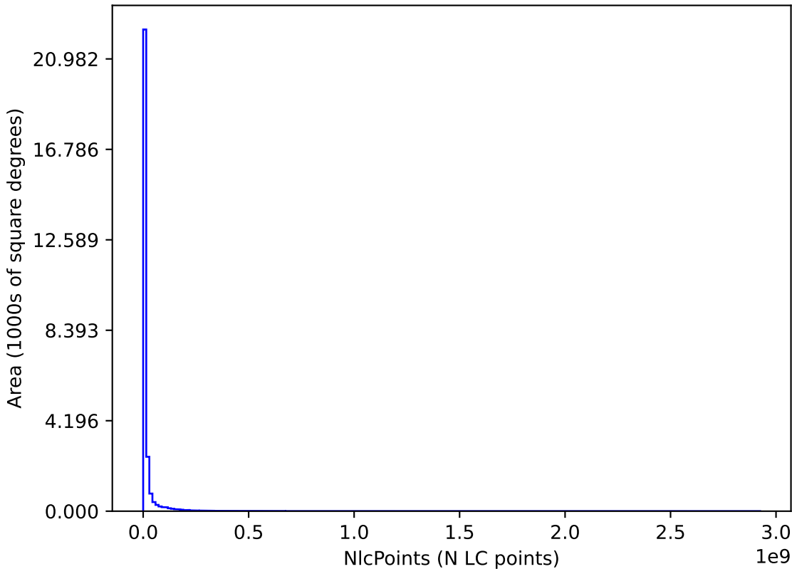
internal_u_expt60_nscale1.1v3.4_10yrs : NlcPoints
