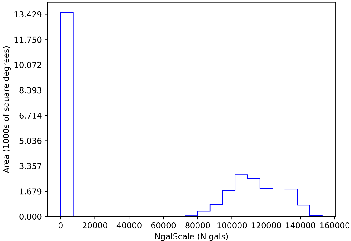
internal_u_expt60_nscale1.1v3.4_10yrs i: NgalScale
