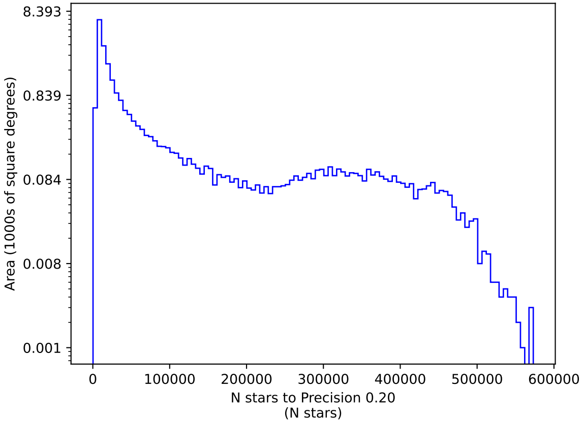
internal_u_expt60_nscale1.1v3.4_10yrs y: N stars to Precision 0.20
