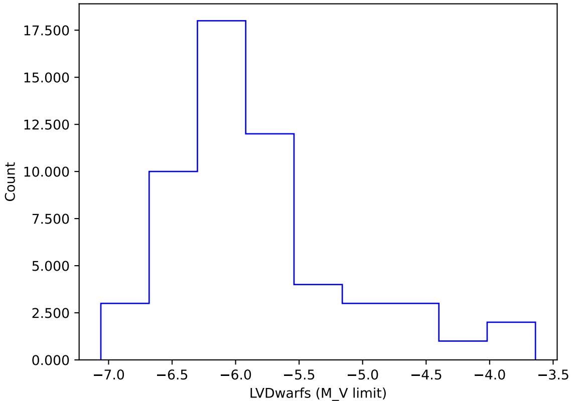
internal_u_expt60_nscale1.1v3.4_10yrs gi: LVDwarfs
